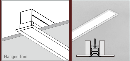
Flanged Trim
